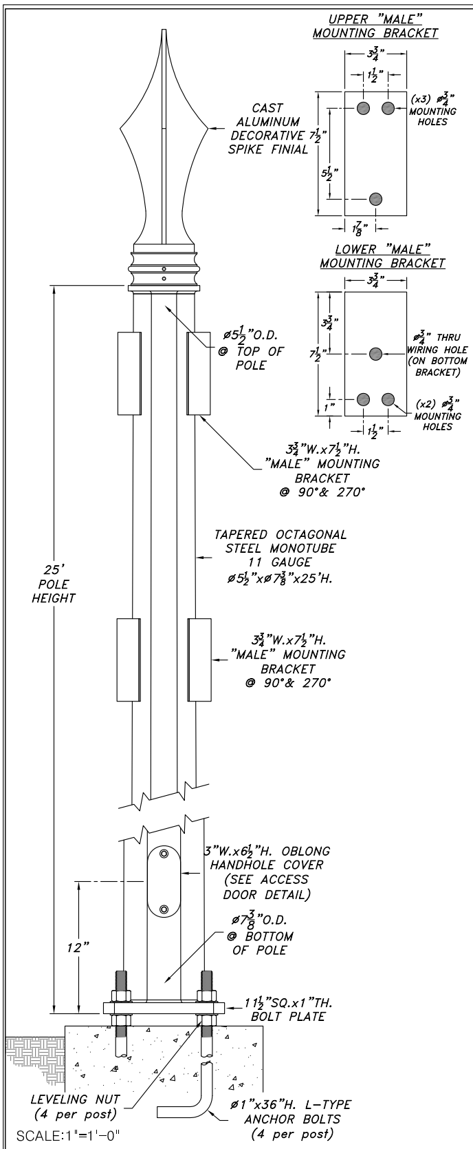
Steel Series-11" Bolt Plate-Tapered Octagonal Steel Pole-25' Height SS-11-OCT-25
